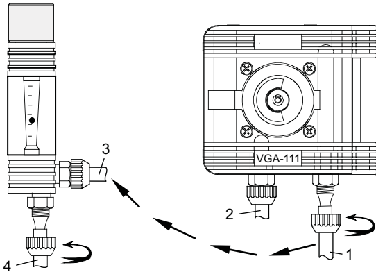
Abb. 11 Anschlüsse
